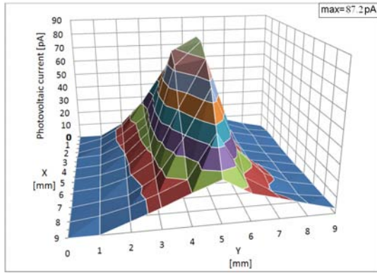
Figure 4. CCP scan at 20°C and 160 mW/cm 2 of illumination.
